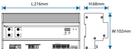
Figure 2. Dimensional Drawing - Front View
