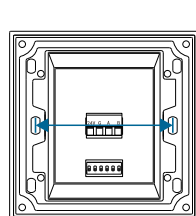
Figure 10.Installation hole position diagram
