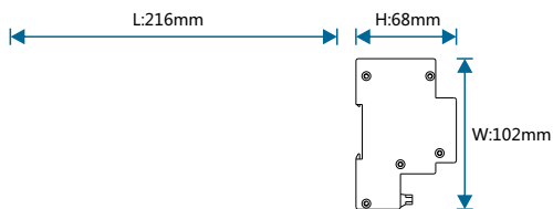
Figure 2. Dimensional Drawing - Front View
